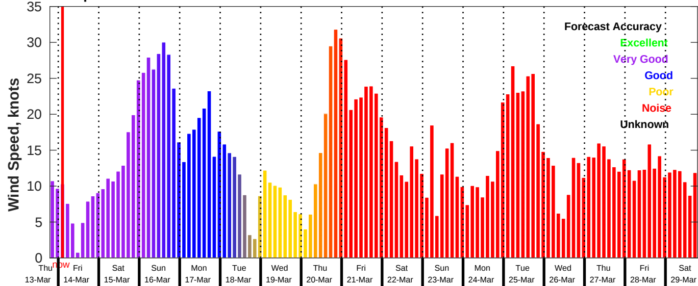
GFS Wind Speed Forecast for NDBC 41004 from 13-Mar-2025 19:00:00 to 29-Mar-2025 19:00:00
