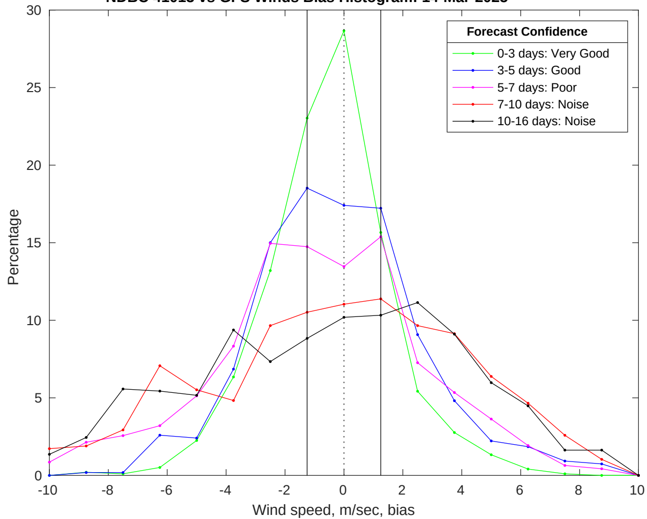
NDBC 41013 vs GFS Winds Bias Histogram: 14-Mar-2025
