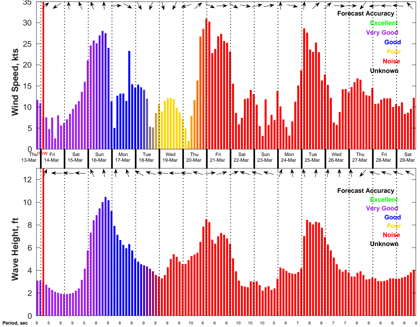
Wind & Wave Forecast for NDBC 41013 from 13-Mar-2025 19:00:00 to 29-Mar-2025 19:00:00
