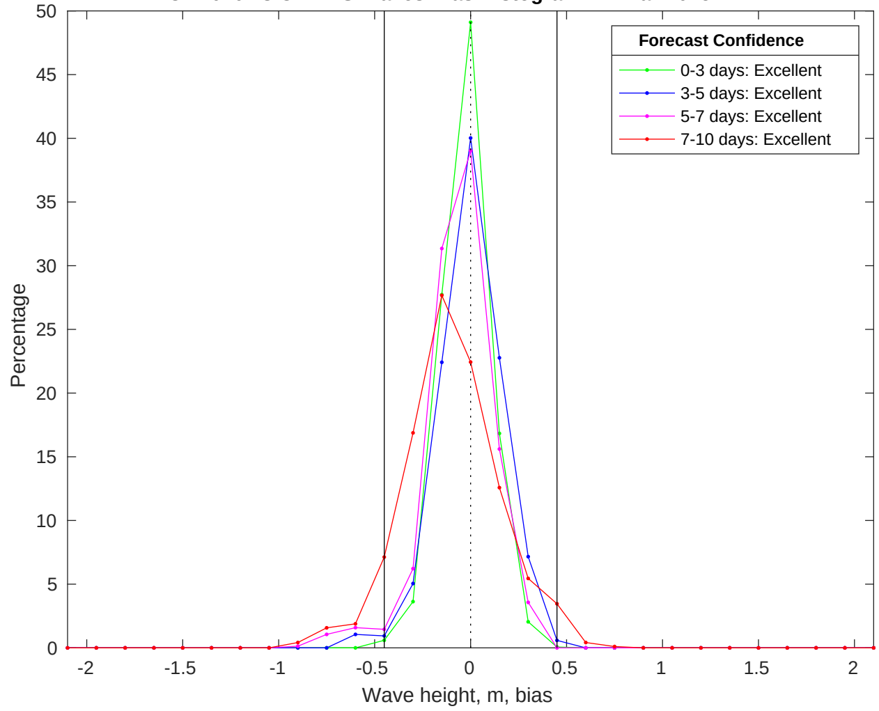
NDBC 41040 vs CMEMS Waves Bias Histogram: 14-Mar-2025
