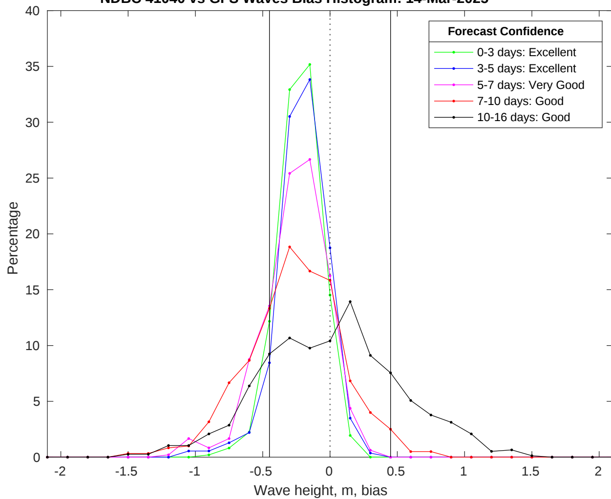
NDBC 41040 vs GFS Waves Bias Histogram: 14-Mar-2025
