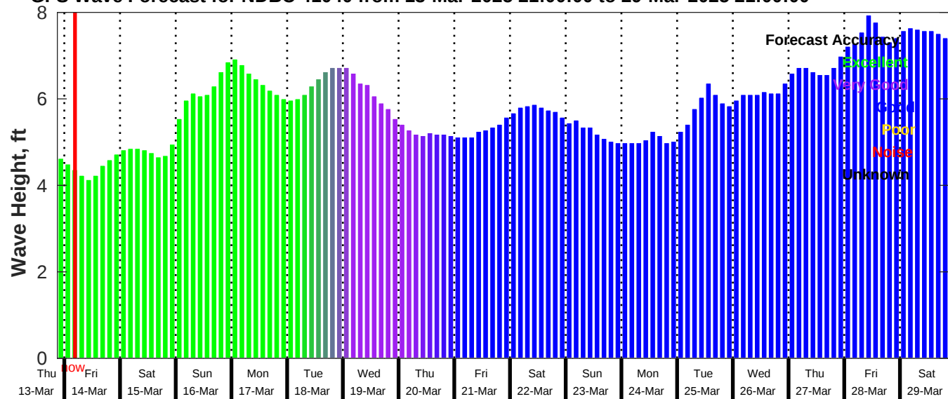
GFS Wave Forecast for NDBC 41040 from 13-Mar-2025 21:00:00 to 29-Mar-2025 21:00:00
