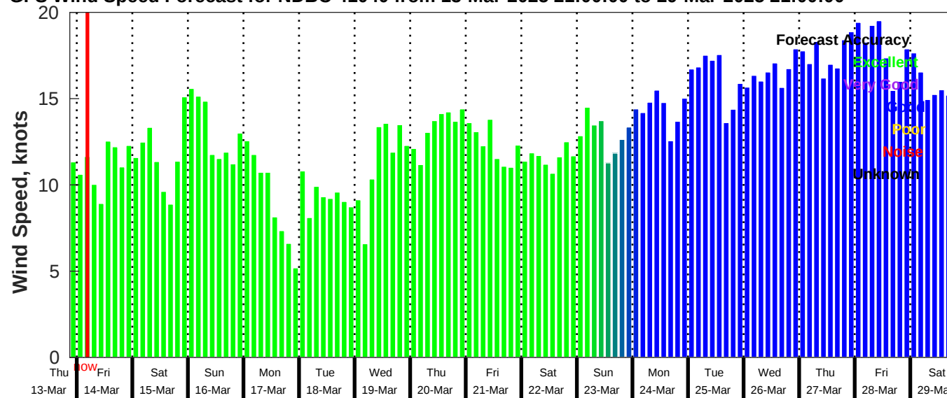
GFS Wind Speed Forecast for NDBC 41040 from 13-Mar-2025 21:00:00 to 29-Mar-2025 21:00:00
