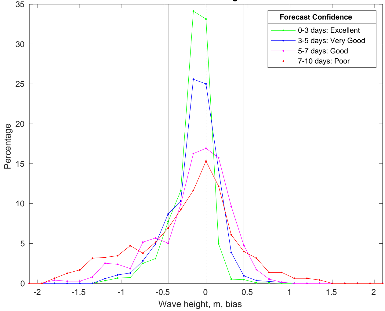
NDBC 42019 vs CMEMS Waves Bias Histogram: 14-Mar-2025
