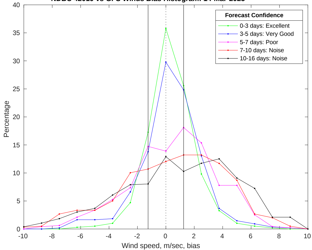
NDBC 42019 vs GFS Winds Bias Histogram: 14-Mar-2025
