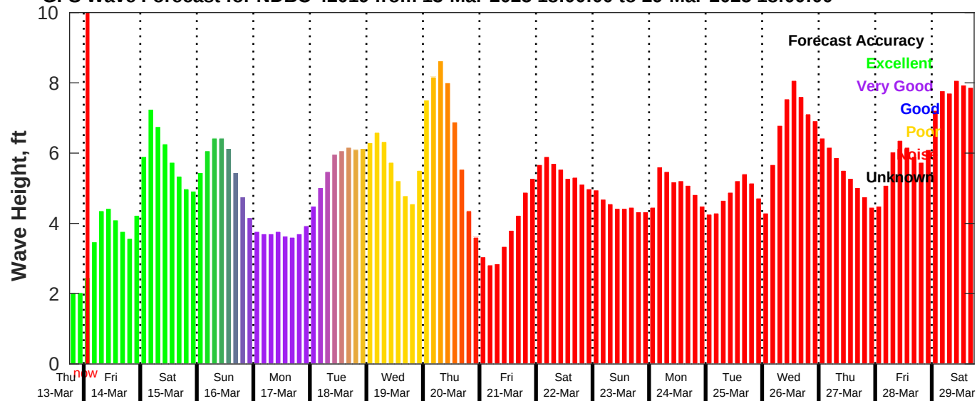
GFS Wave Forecast for NDBC 42019 from 13-Mar-2025 18:00:00 to 29-Mar-2025 18:00:00
