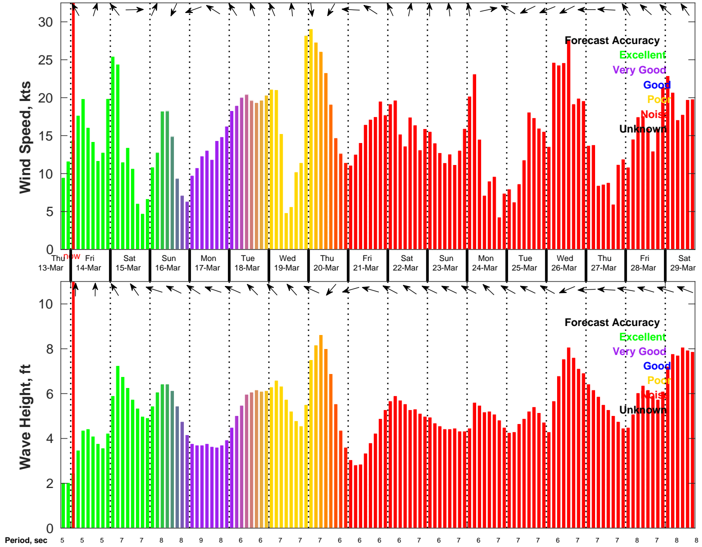
Wind & Wave Forecast for NDBC 42019 from 13-Mar-2025 18:00:00 to 29-Mar-2025 18:00:00
