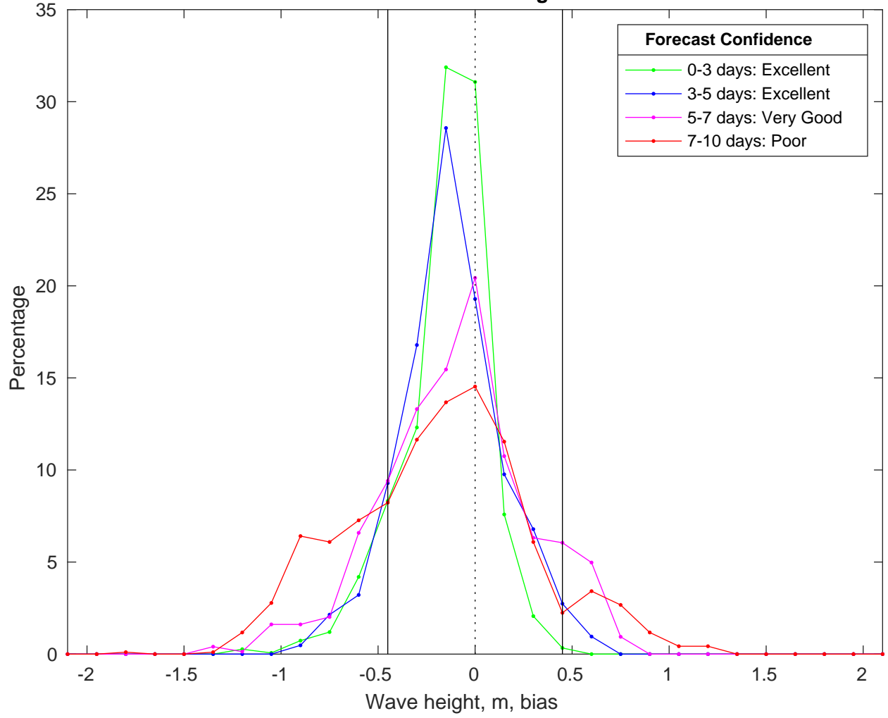
NDBC 42020 vs CMEMS Waves Bias Histogram: 14-Mar-2025
