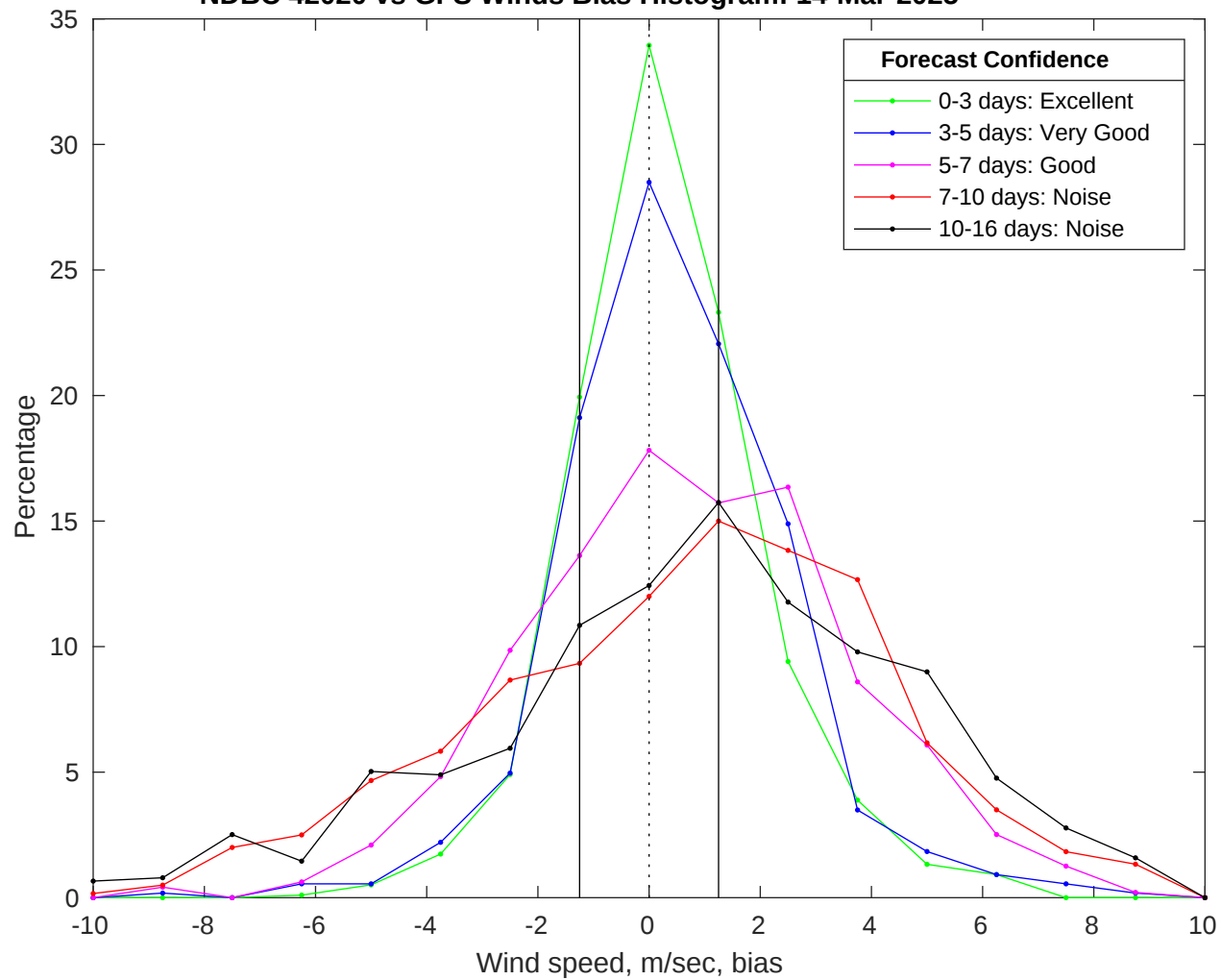
NDBC 42020 vs GFS Winds Bias Histogram: 14-Mar-2025
