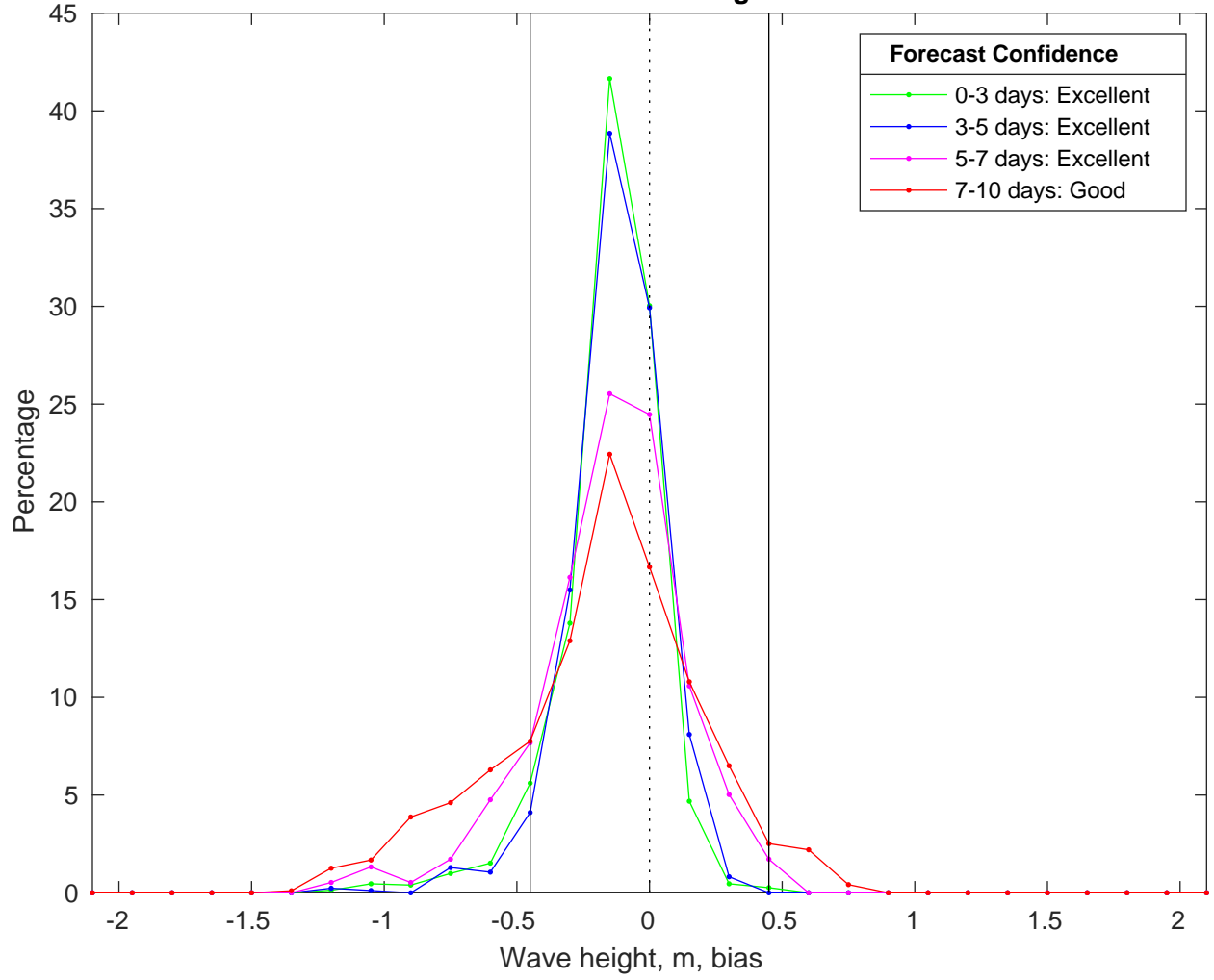
NDBC 42035 vs CMEMS Waves Bias Histogram: 14-Mar-2025
