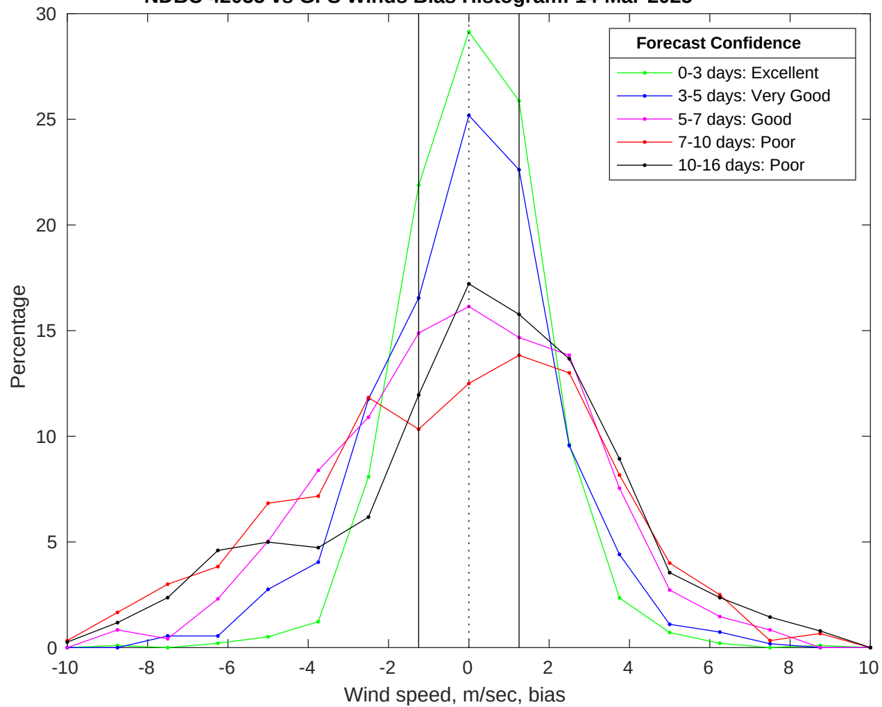
NDBC 42035 vs GFS Winds Bias Histogram: 14-Mar-2025
