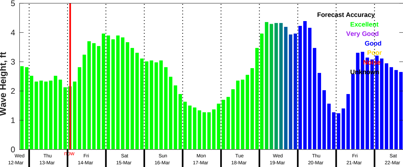
CMEMS Wave Forecast for NDBC 42035 from 12-Mar-2025 18:00:00 to 22-Mar-2025 18:00:00
