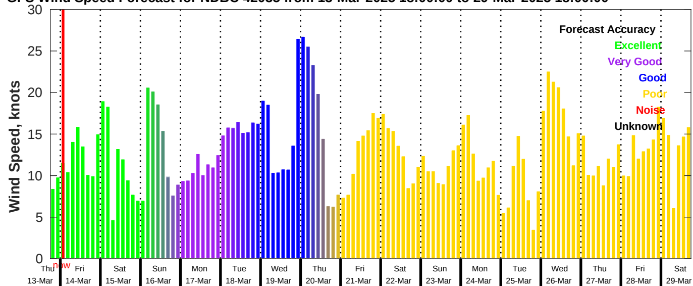
GFS Wind Speed Forecast for NDBC 42035 from 13-Mar-2025 18:00:00 to 29-Mar-2025 18:00:00
