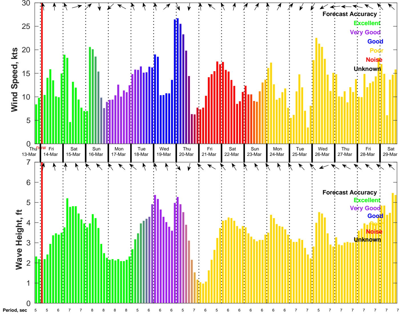
Wind & Wave Forecast for NDBC 42035 from 13-Mar-2025 18:00:00 to 29-Mar-2025 18:00:00
