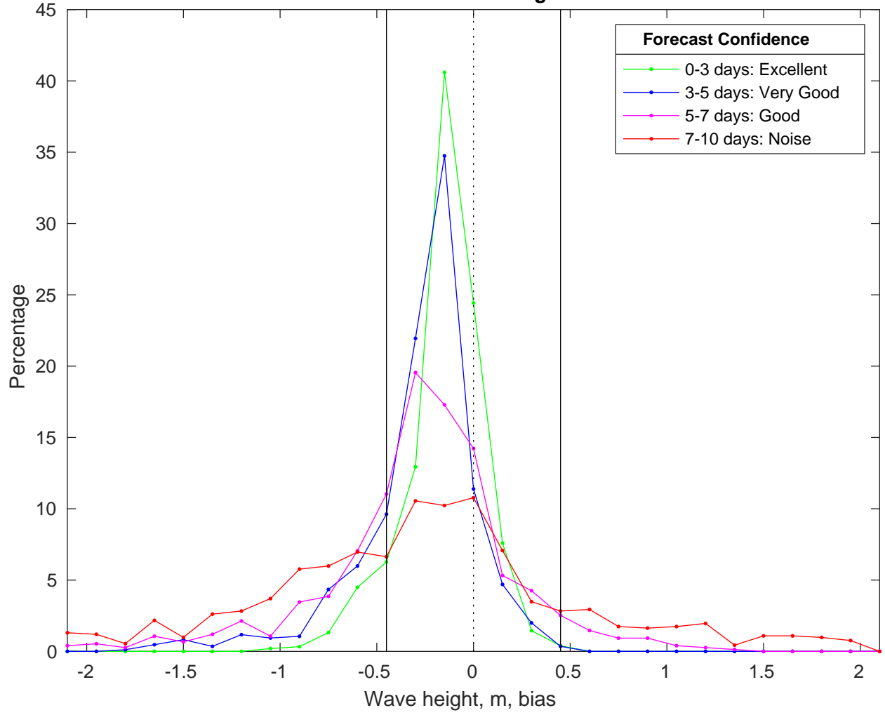
NDBC 42036 vs CMEMS Waves Bias Histogram: 14-Mar-2025
