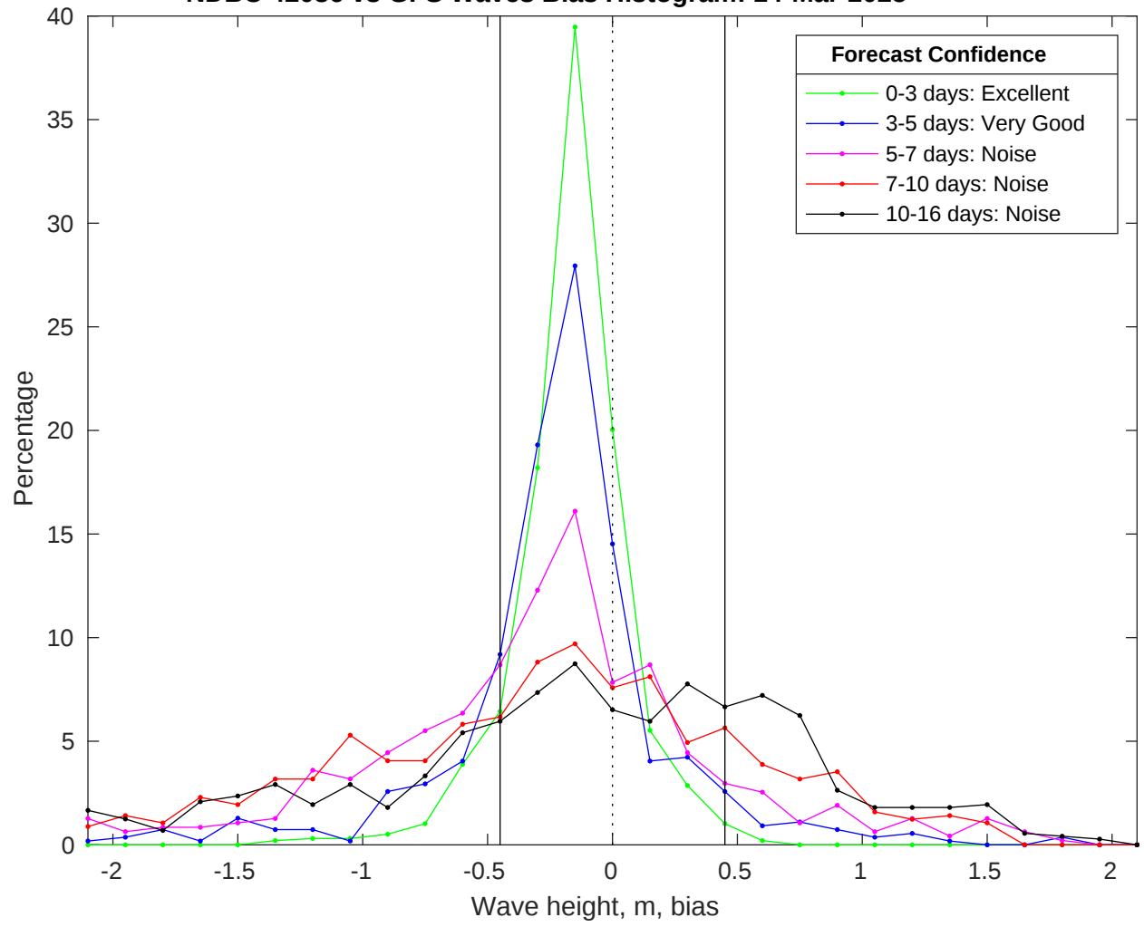
NDBC 42036 vs GFS Waves Bias Histogram: 14-Mar-2025
