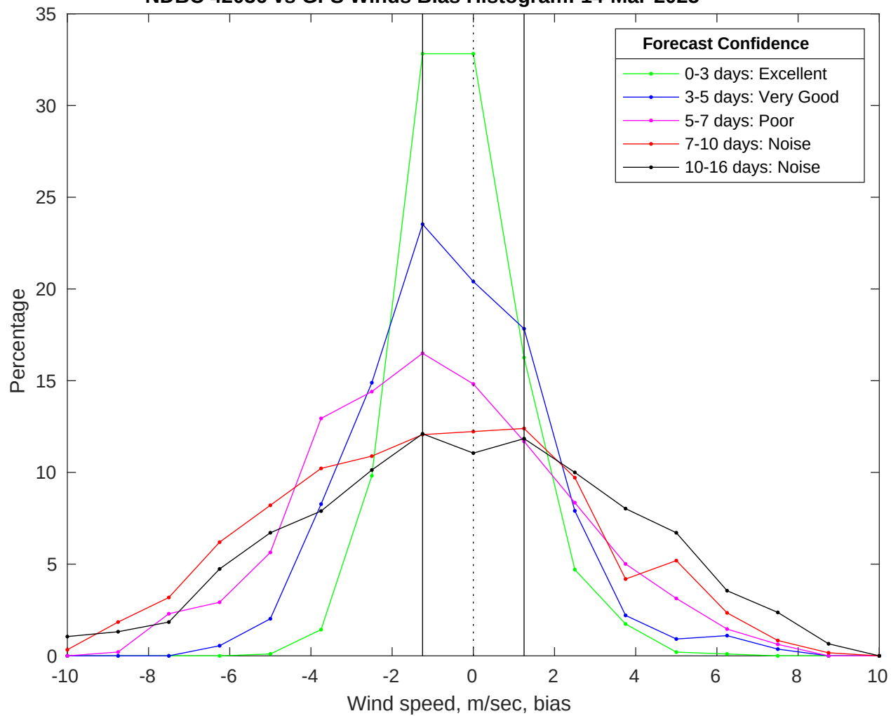
NDBC 42036 vs GFS Winds Bias Histogram: 14-Mar-2025
