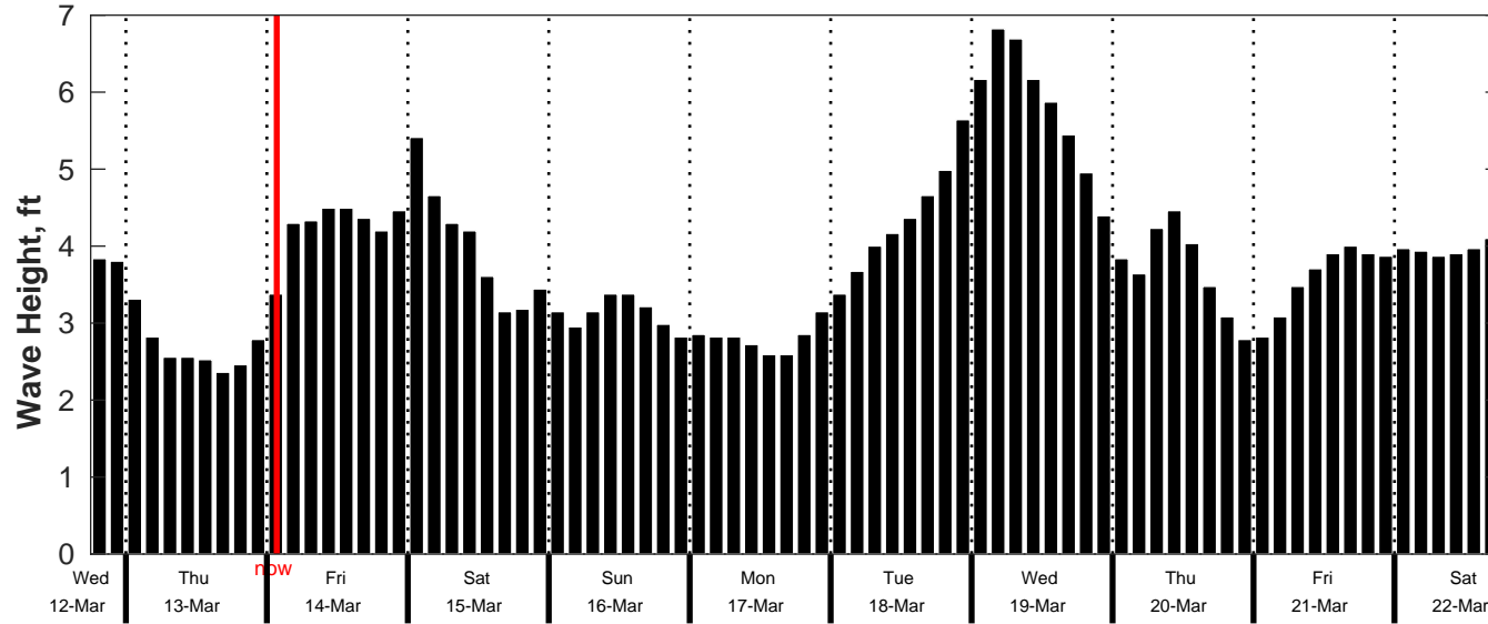
CMEMS Wave Forecast for NDBC 42092 from 12-Mar-2025 18:00:00 to 22-Mar-2025 18:00:00
