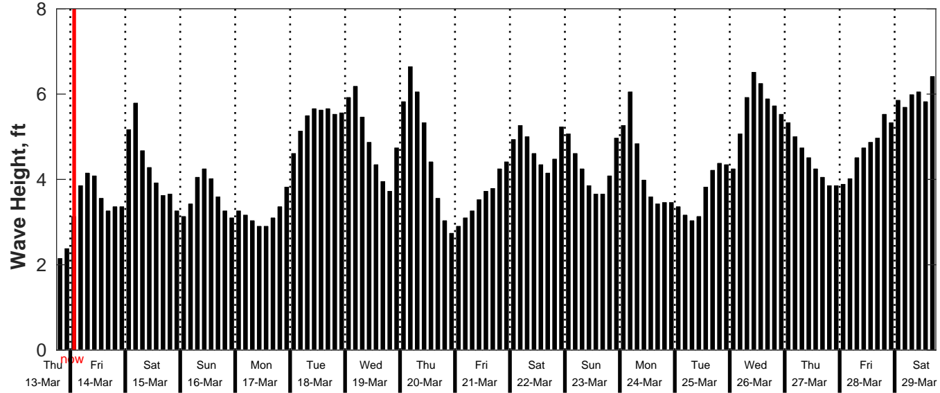
GFS Wave Forecast for NDBC 42092 from 13-Mar-2025 18:00:00 to 29-Mar-2025 18:00:00
