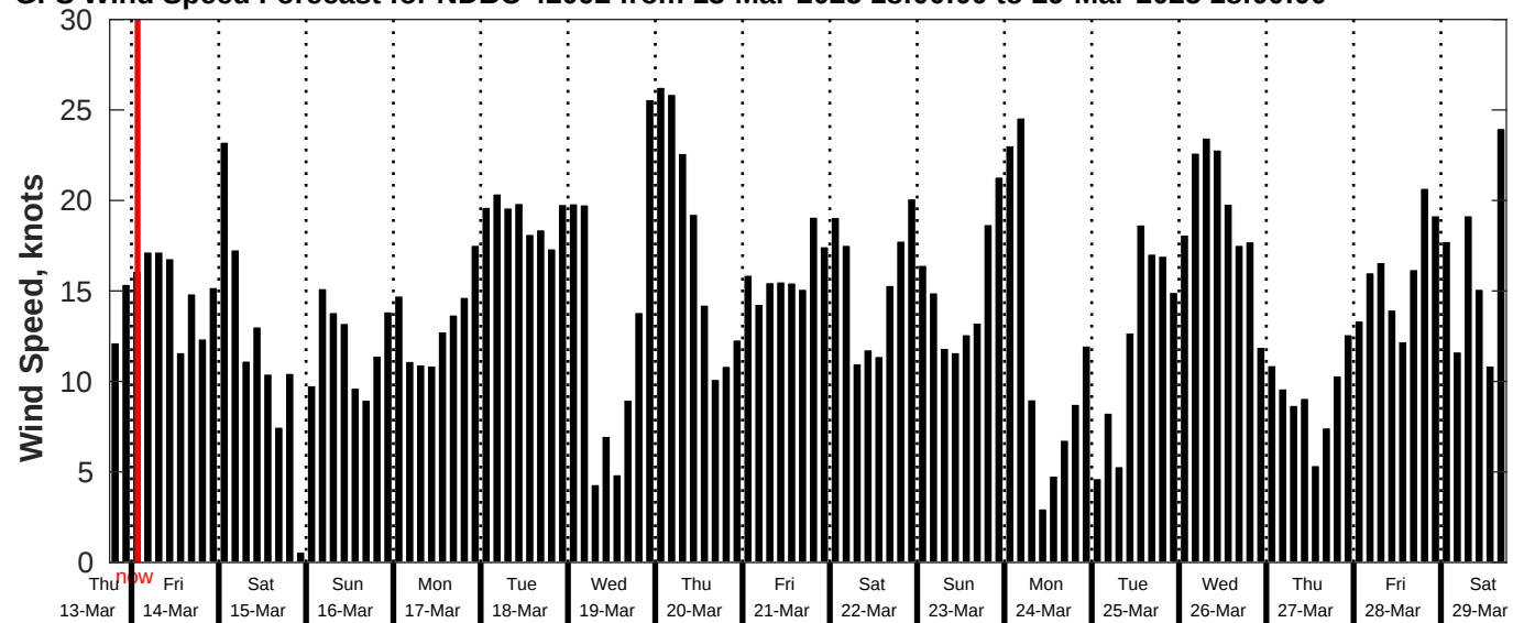
GFS Wind Speed Forecast for NDBC 42092 from 13-Mar-2025 18:00:00 to 29-Mar-2025 18:00:00
