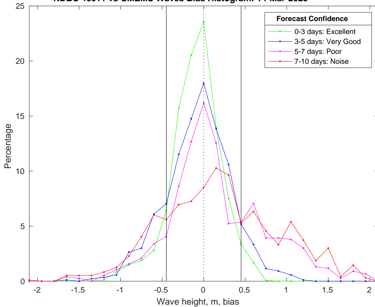
NDBC 46011 vs CMEMS Waves Bias Histogram: 14-Mar-2025
