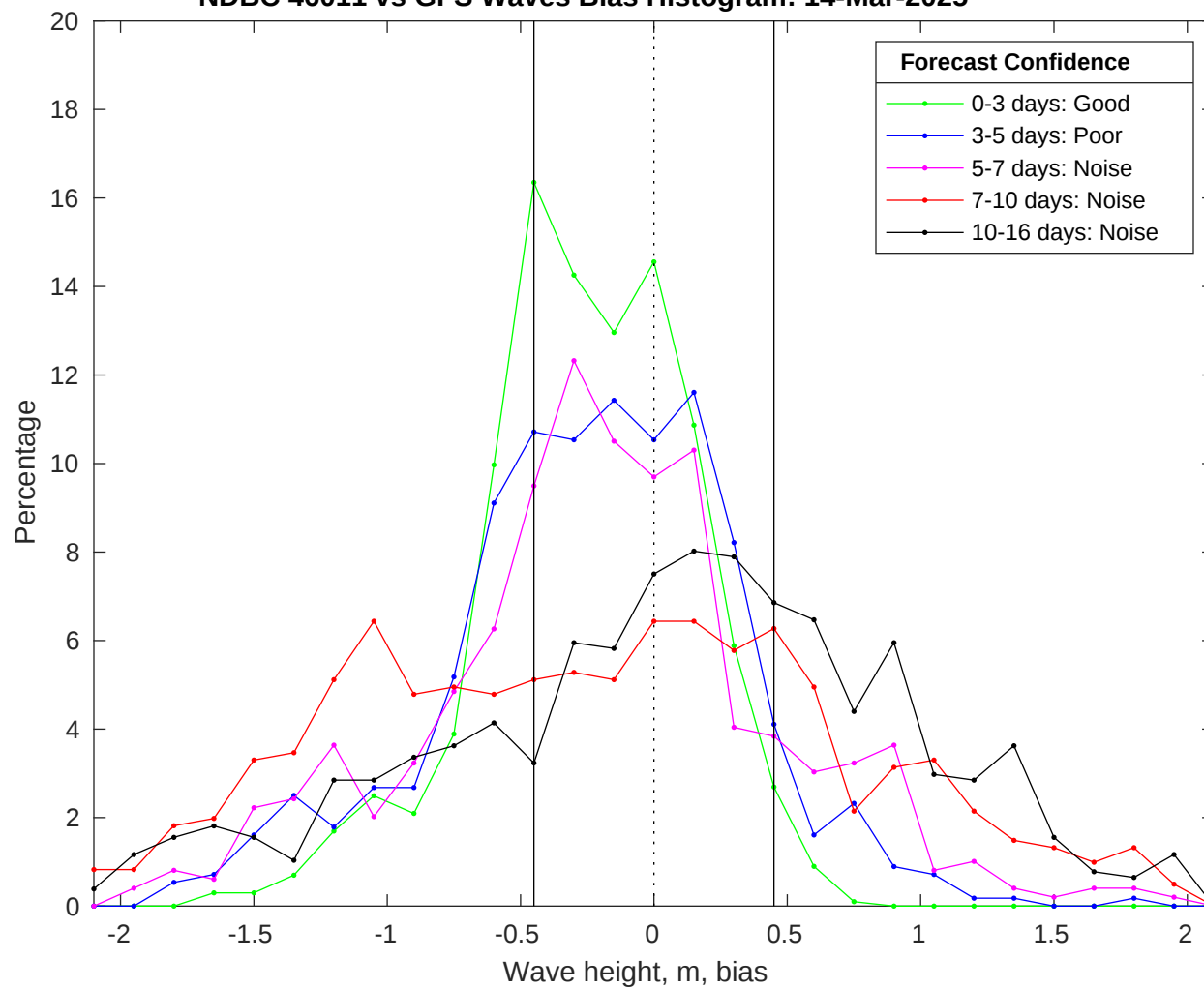
NDBC 46011 vs GFS Waves Bias Histogram: 14-Mar-2025
