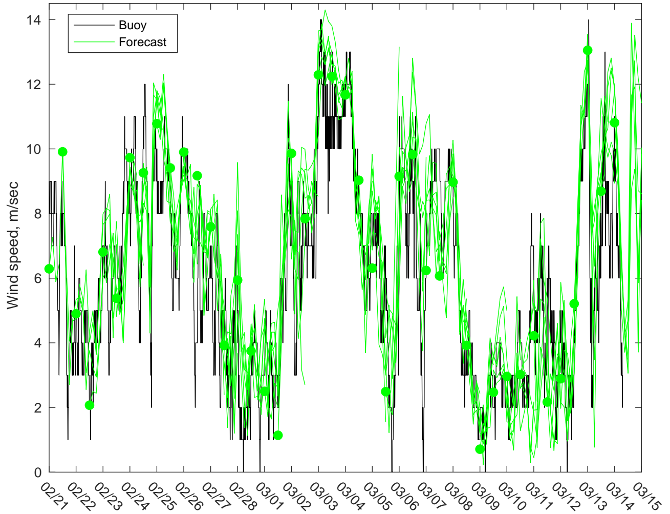
NDBC 46011 vs GFS Winds: 0 to 3 day forecast
