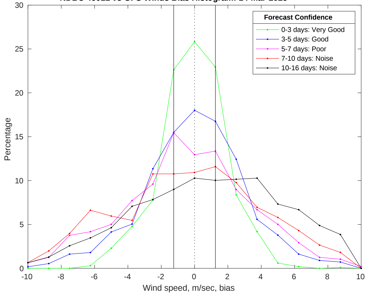
NDBC 46011 vs GFS Winds Bias Histogram: 14-Mar-2025
