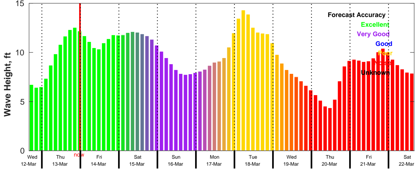
CMEMS Wave Forecast for NDBC 46011 from 12-Mar-2025 16:00:00 to 22-Mar-2025 16:00:00
