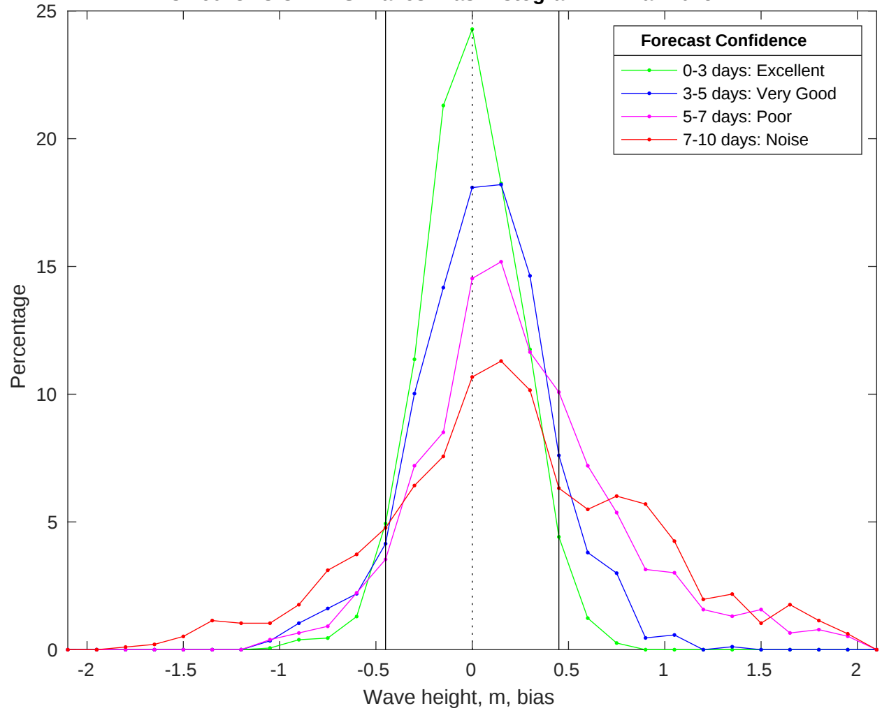
NDBC 46028 vs CMEMS Waves Bias Histogram: 14-Mar-2025
