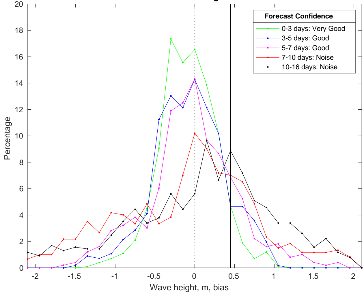
NDBC 46028 vs GFS Waves Bias Histogram: 14-Mar-2025
