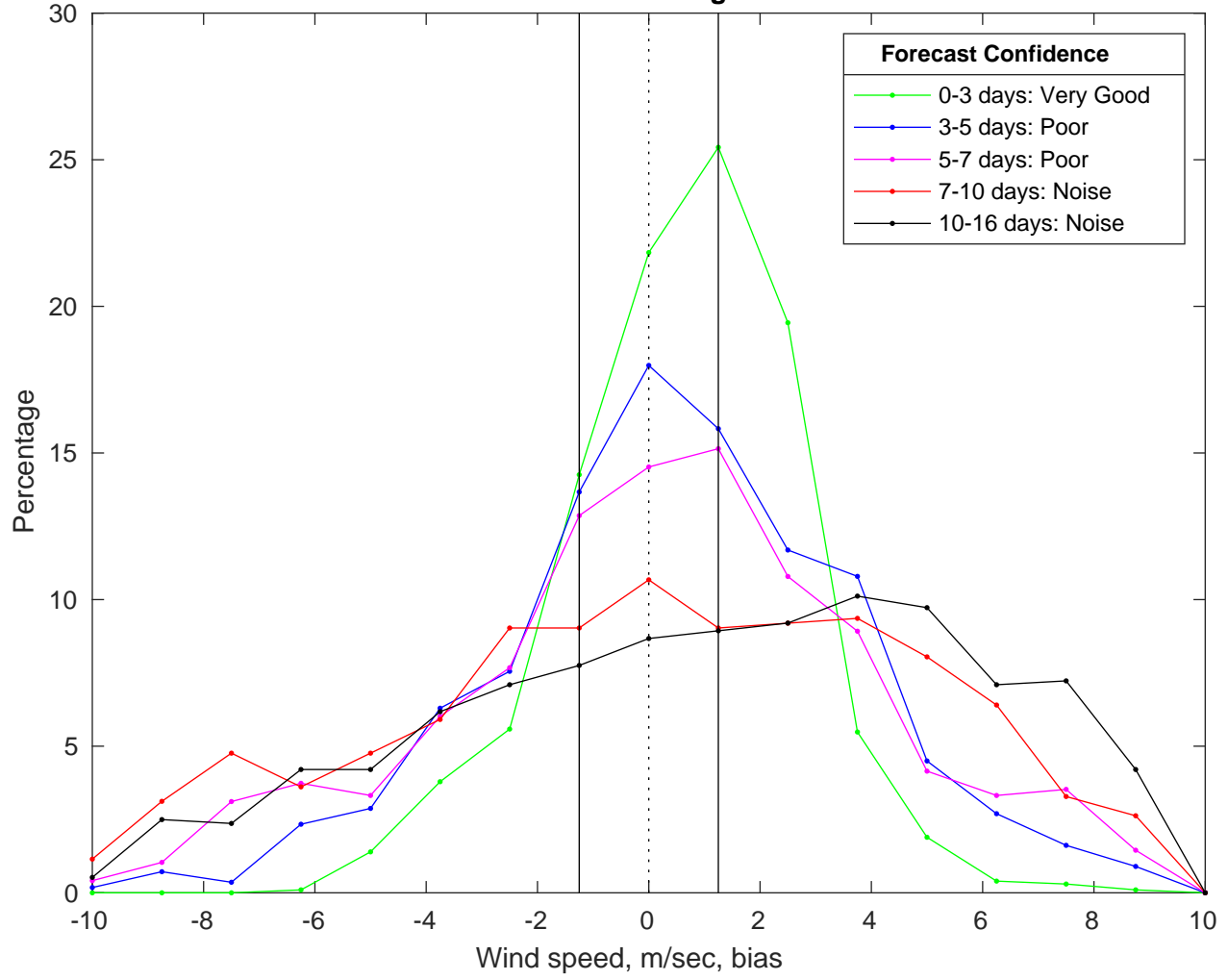
NDBC 46028 vs GFS Winds Bias Histogram: 14-Mar-2025
