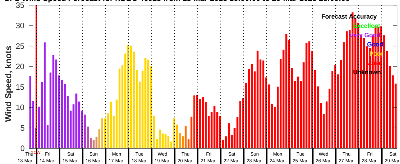
GFS Wind Speed Forecast for NDBC 46028 from 13-Mar-2025 16:00:00 to 29-Mar-2025 16:00:00
