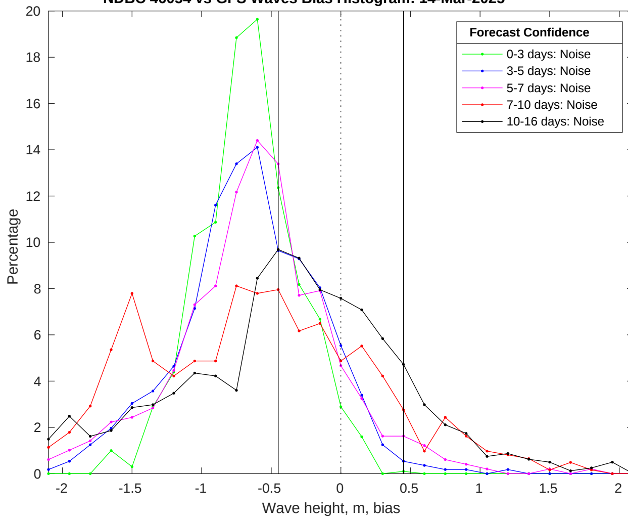
NDBC 46054 vs GFS Waves Bias Histogram: 14-Mar-2025
