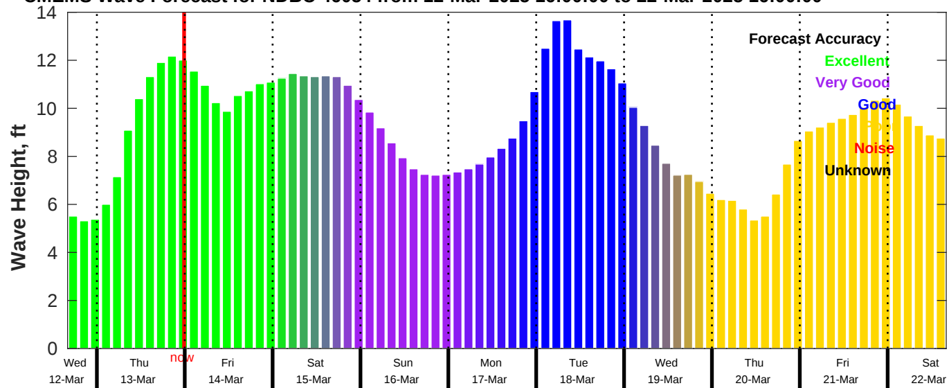
CMEMS Wave Forecast for NDBC 46054 from 12-Mar-2025 16:00:00 to 22-Mar-2025 16:00:00
