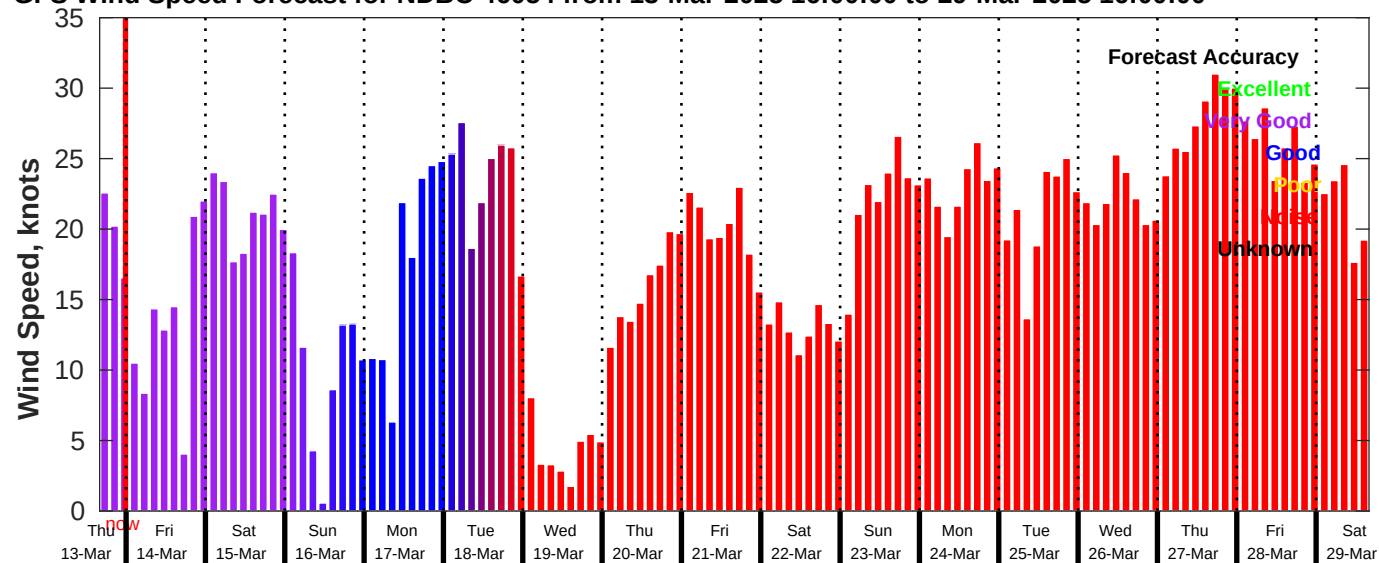
GFS Wind Speed Forecast for NDBC 46054 from 13-Mar-2025 16:00:00 to 29-Mar-2025 16:00:00
