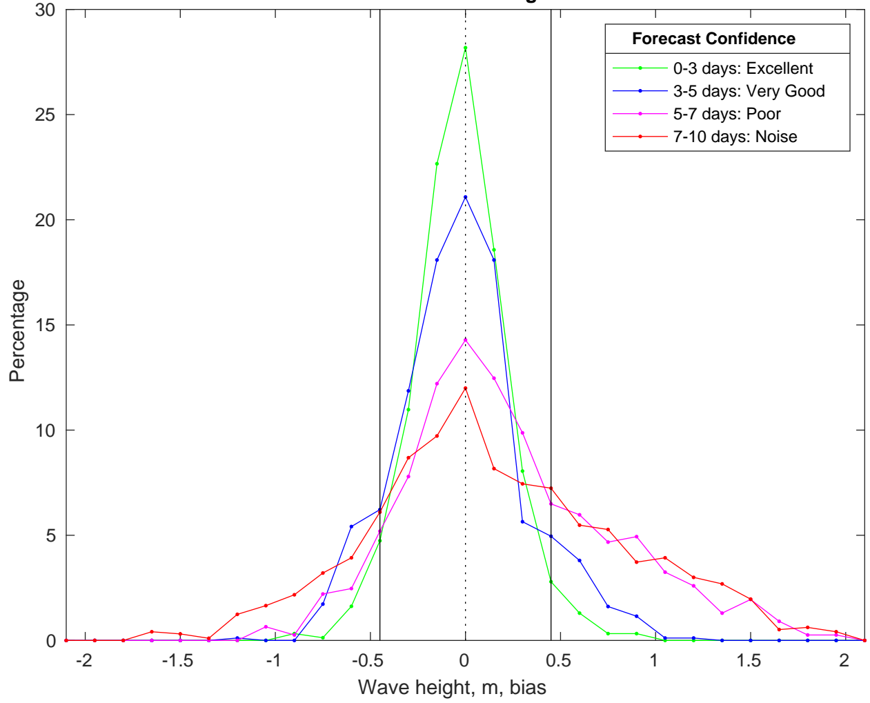
NDBC 46069 vs CMEMS Waves Bias Histogram: 14-Mar-2025
