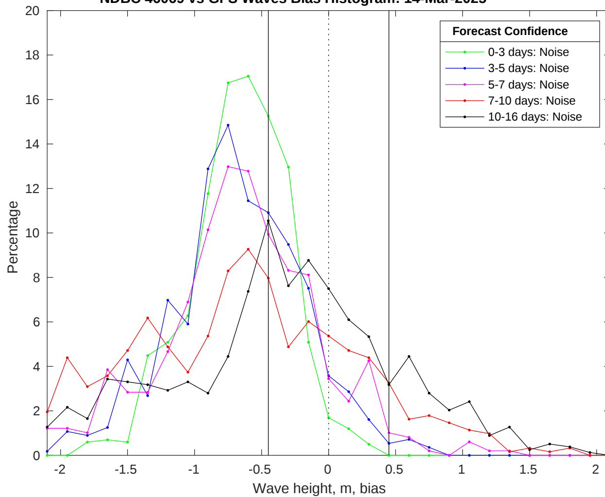
NDBC 46069 vs GFS Waves Bias Histogram: 14-Mar-2025
