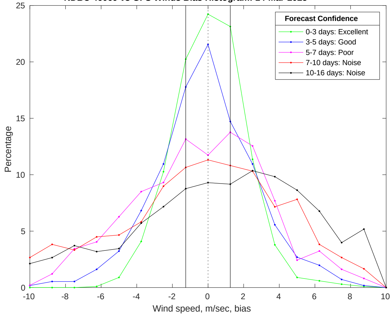
NDBC 46069 vs GFS Winds Bias Histogram: 14-Mar-2025
