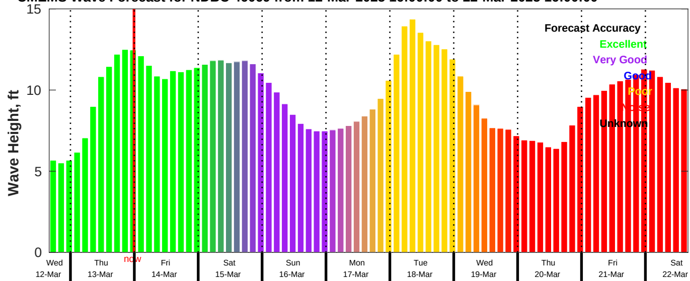
CMEMS Wave Forecast for NDBC 46069 from 12-Mar-2025 16:00:00 to 22-Mar-2025 16:00:00
