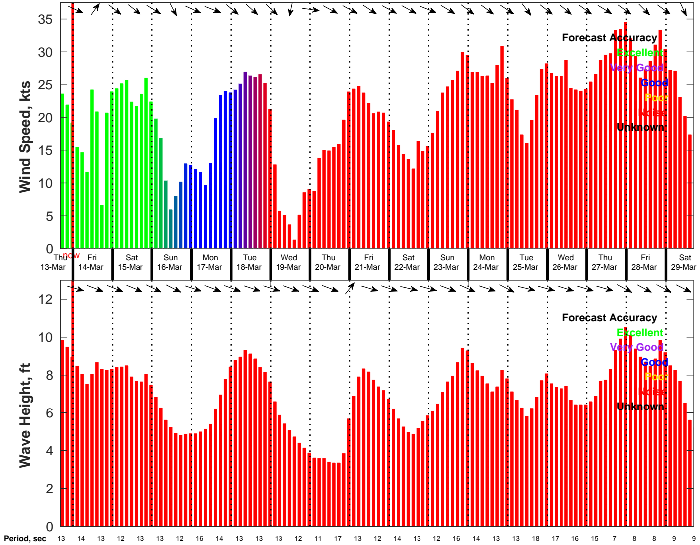
Wind & Wave Forecast for NDBC 46069 from 13-Mar-2025 16:00:00 to 29-Mar-2025 16:00:00
