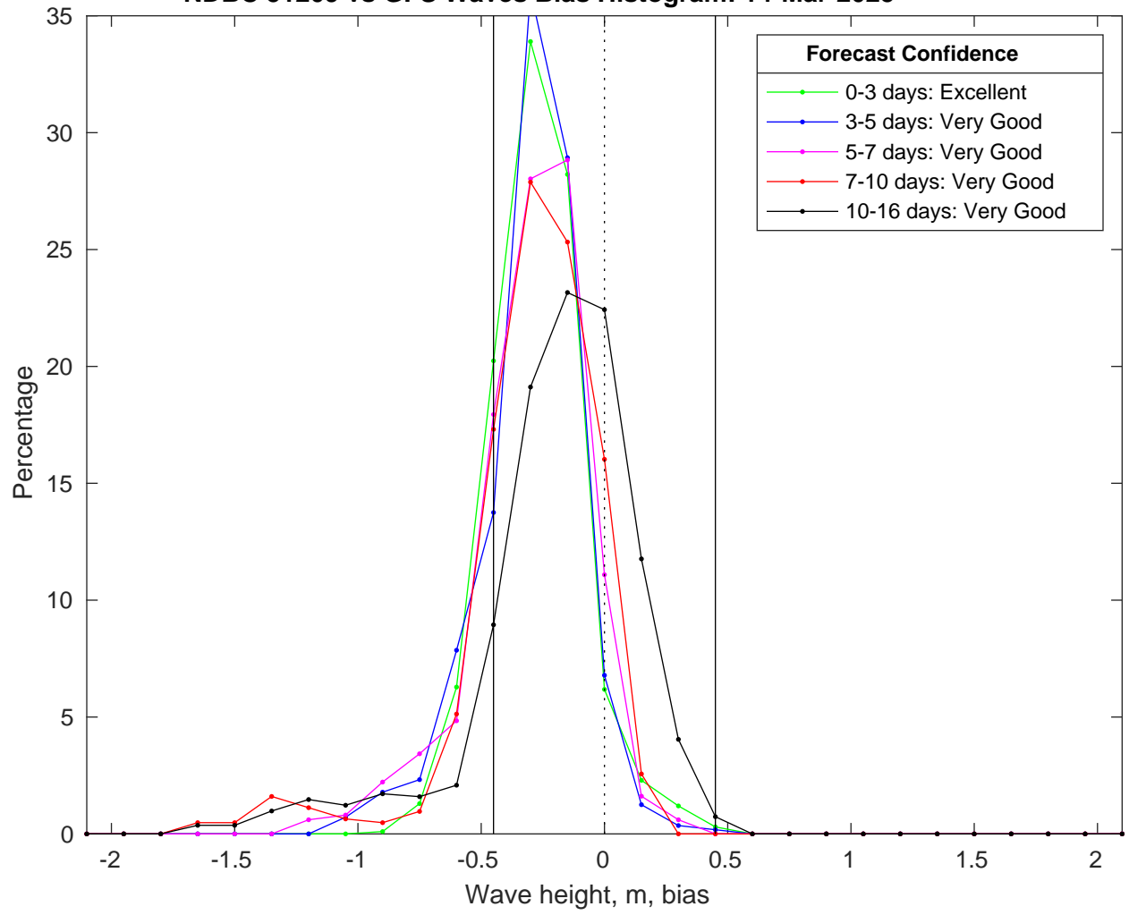
NDBC 51209 vs GFS Waves Bias Histogram: 14-Mar-2025
