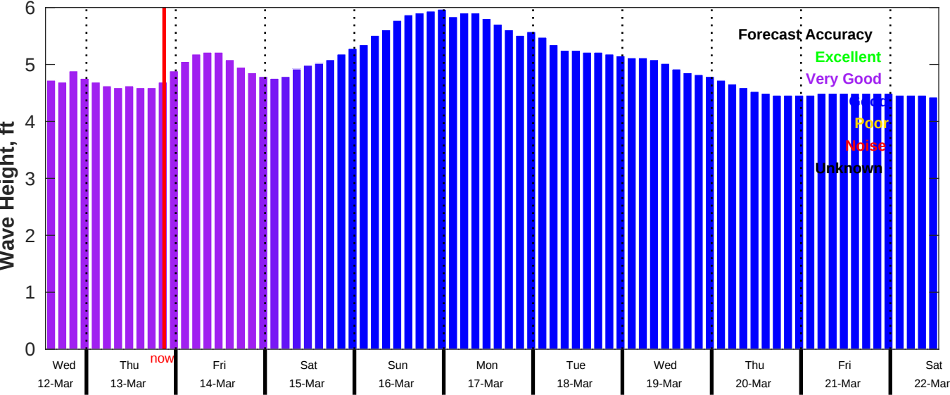
CMEMS Wave Forecast for NDBC 51209 from 12-Mar-2025 13:00:00 to 22-Mar-2025 13:00:00
