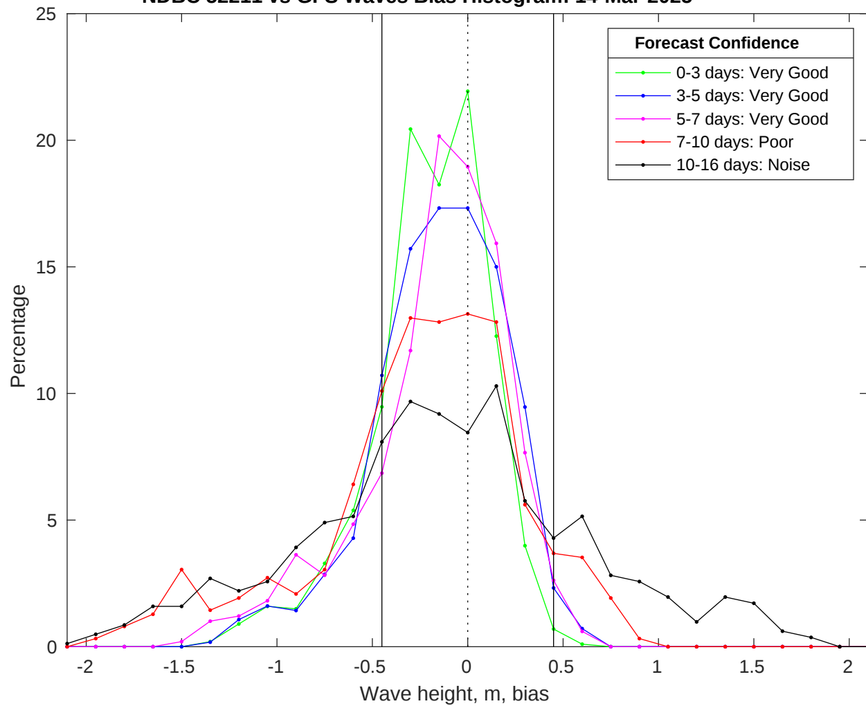
NDBC 52211 vs GFS Waves Bias Histogram: 14-Mar-2025
