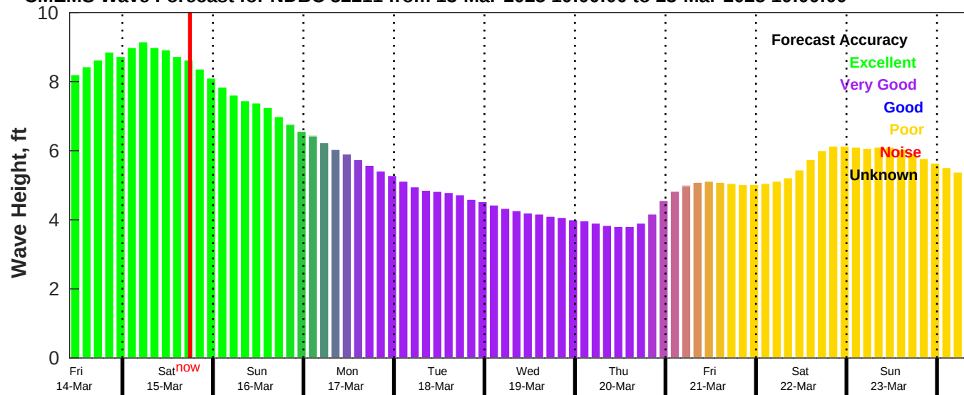
CMEMS Wave Forecast for NDBC 52211 from 13-Mar-2025 10:00:00 to 23-Mar-2025 10:00:00
