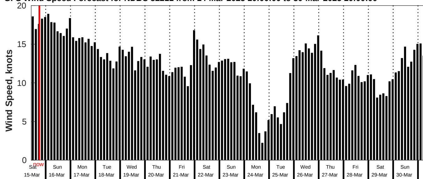
GFS Wind Speed Forecast for NDBC 52211 from 14-Mar-2025 10:00:00 to 30-Mar-2025 10:00:00
