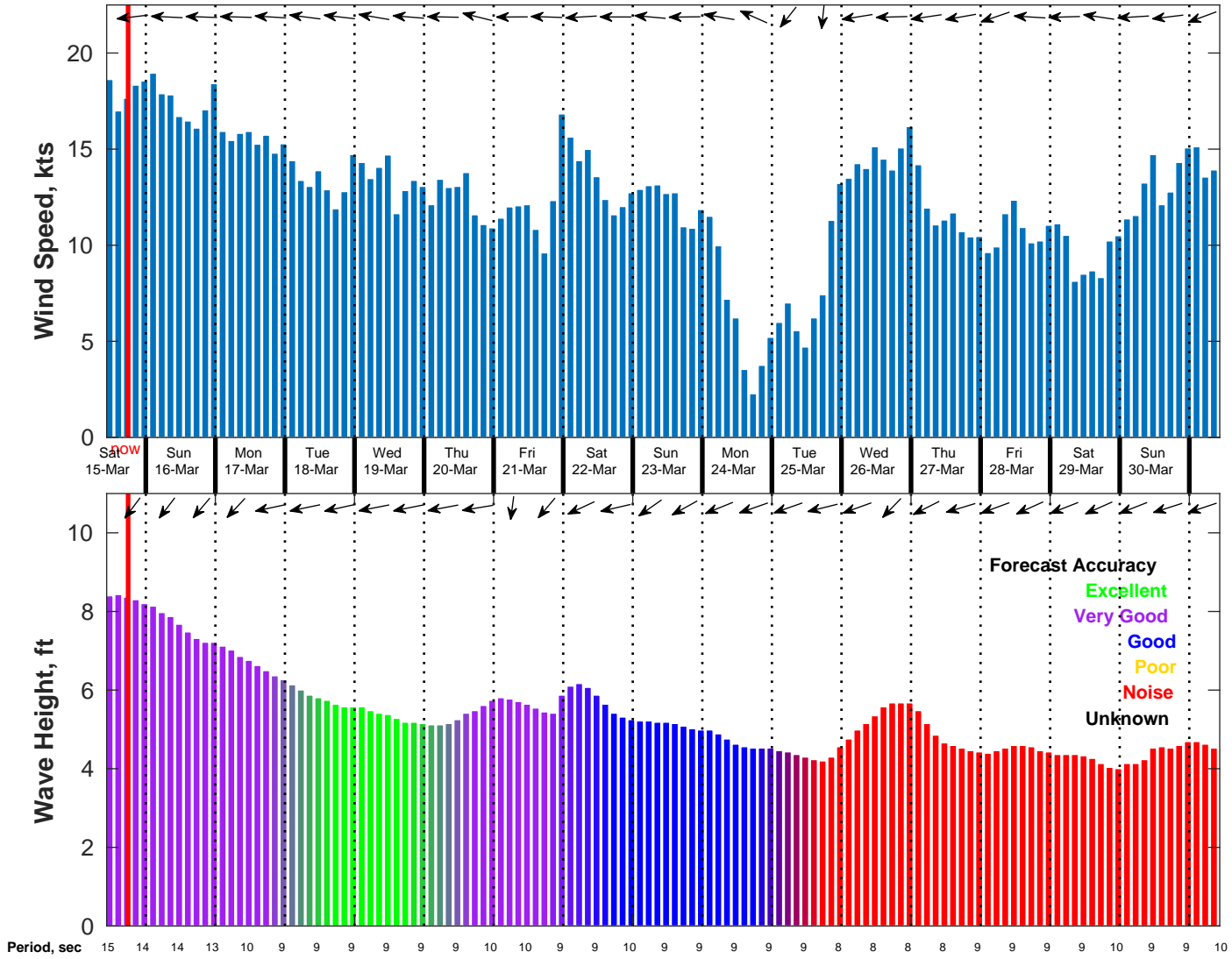
Wind & Wave Forecast for NDBC 52211 from 14-Mar-2025 10:00:00 to 30-Mar-2025 10:00:00
