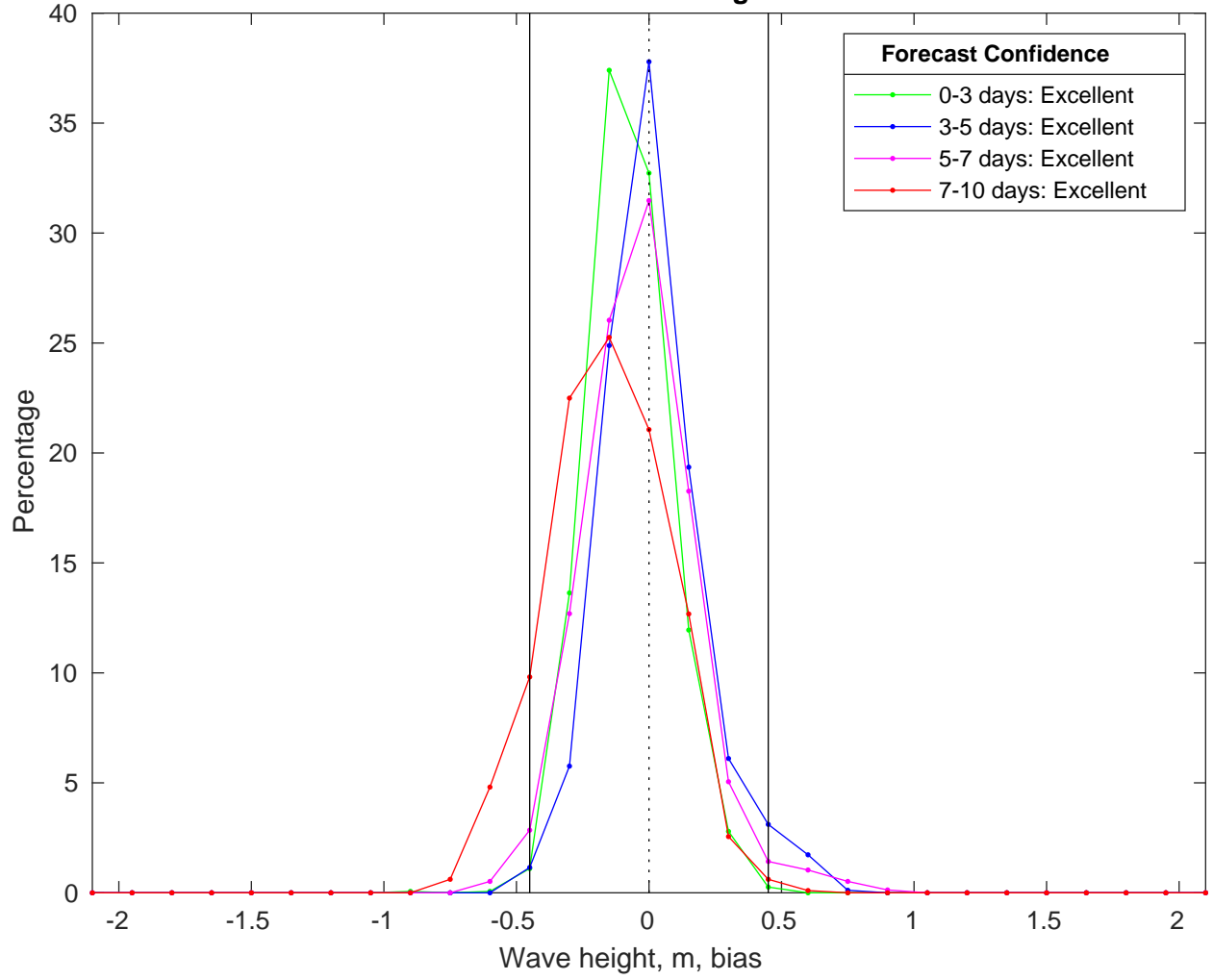
NDBC 52212 vs CMEMS Waves Bias Histogram: 14-Mar-2025
