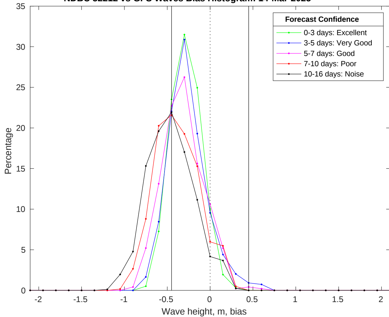
NDBC 52212 vs GFS Waves Bias Histogram: 14-Mar-2025
