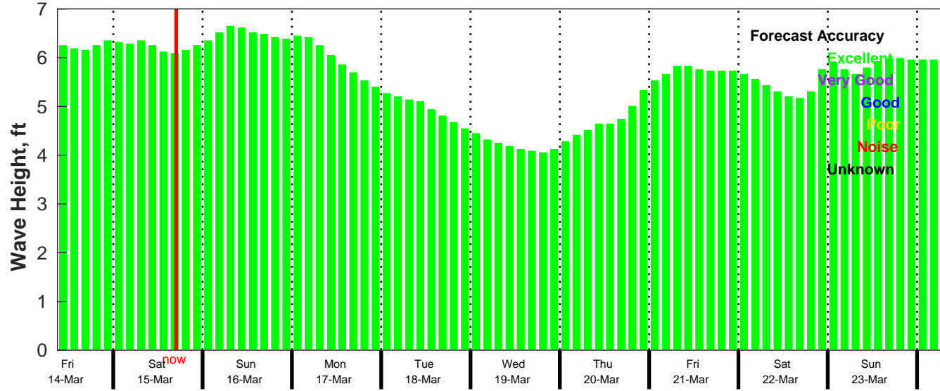
CMEMS Wave Forecast for NDBC 52212 from 13-Mar-2025 09:00:00 to 23-Mar-2025 09:00:00
